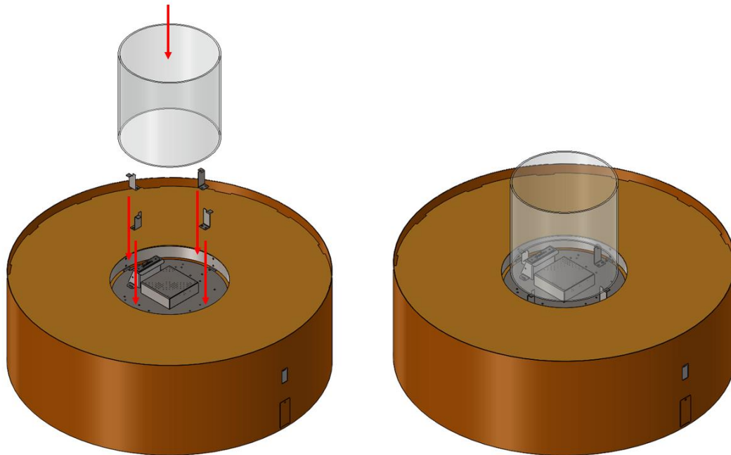
Fig 4 – Glass cylinder installation
