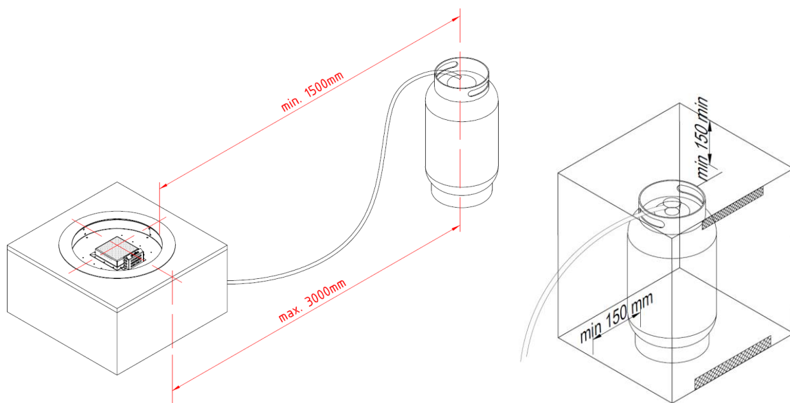
Fig 5 – Gas cylinder distnace
