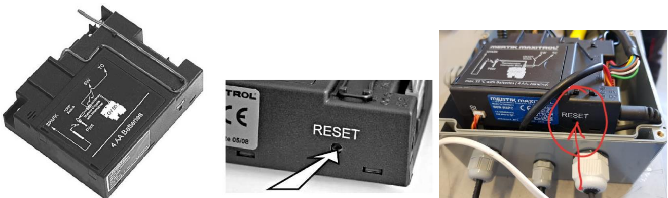
Fig 7: Receiver "RESET" button
